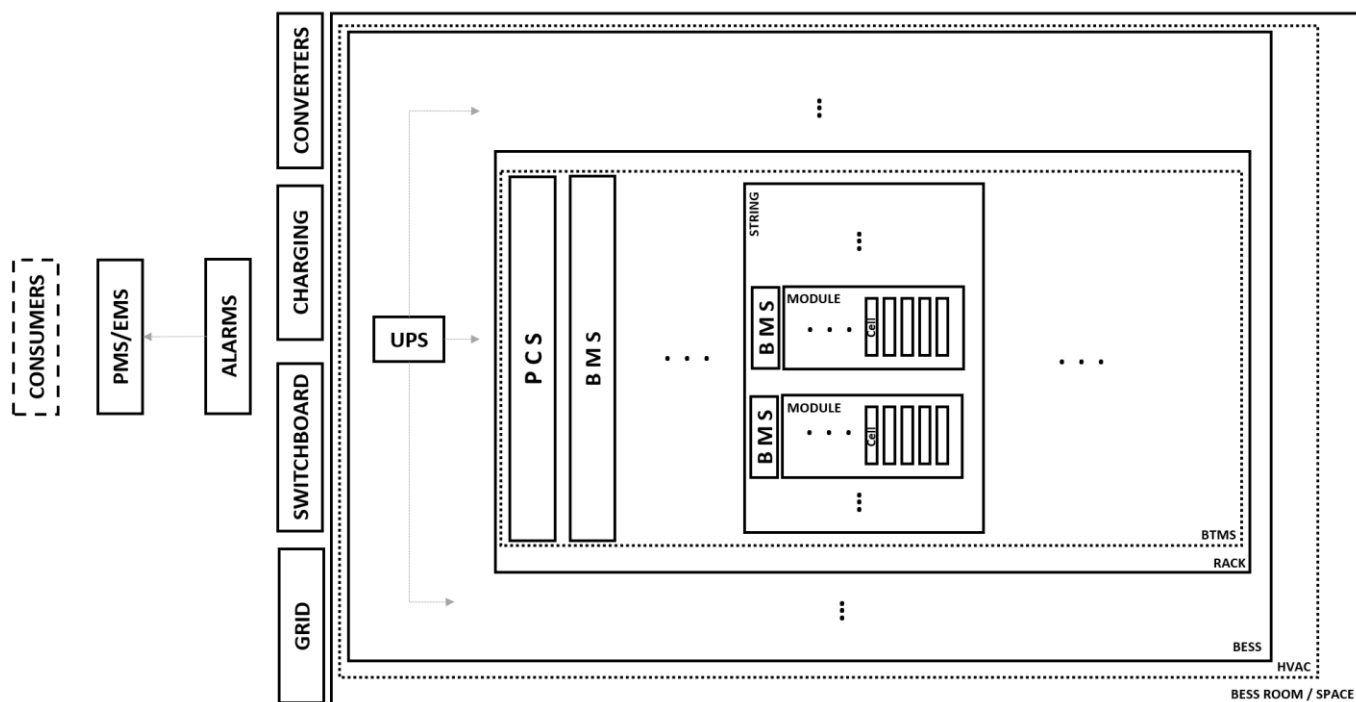
Schematics of BESS boundaries
